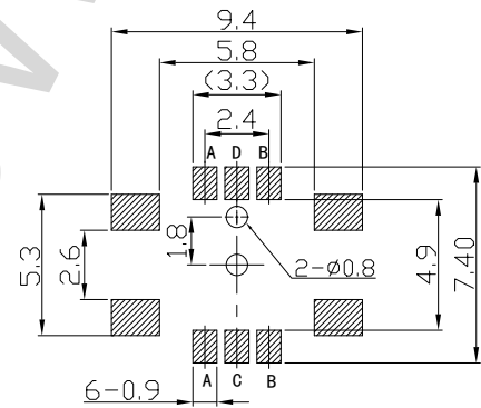
P. C. B Mounting Holes Detail
